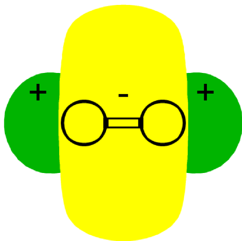
Bonding MO, \sigma_{2pz}
